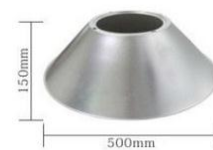
120° reflector
